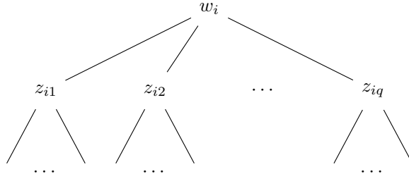
Figure 5: A less simple non-tautology
