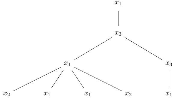
Figure 2: A general implication tree representing the Boolean function x_1 \vee \bar{x}_3 .
