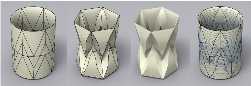
Fig. 14. Interactive modeling of a cylindrical curved-crease sculpture. During modeling we maintain the property of unfoldability onto a cylinder (this is implemented via cutting the surface open and requiring a planar development with periodicity). From left: a user’s initial sketch of the combinatorics, the final sculpture with and without patch boundaries, and the cylindrical development.
