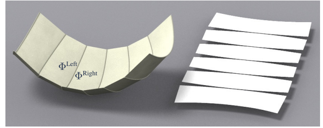
Fig. 7. Here, unfolding neighbouring strips \Phi^{\text{Left}}, \Phi^{\text{Right}} maps their common boundary to planar curves which are mirror reflections of each other. This “geodesic” property makes the developments of strips straighter, which is useful for materials like wood [Meredith and Kotronis 2012].
