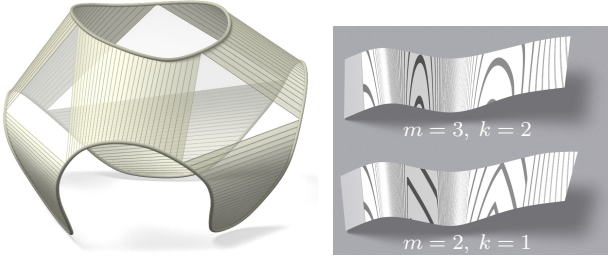
Fig. 3. Developables decompose into planar pieces and ruled patches. Curvature continuity is relevant for surface quality since it becomes visible in reflection patterns. The right hand images show spline developables of varying degree m and smoothness C^k .
