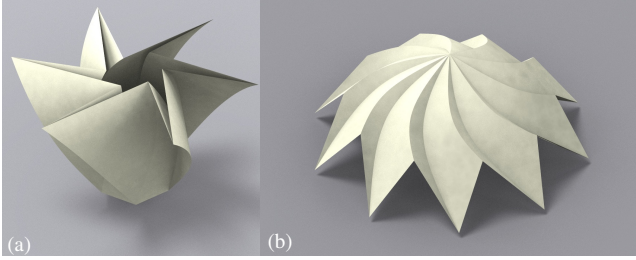
Fig. 6. Shapes foldable from a single sheet of paper consist of ruled developables. Secondly, smooth creases enjoy the “curved fold” property, and thirdly the angle sum around each vertex equals 2\pi . These three conditions are sufficient for local developability.
