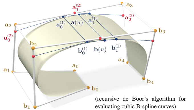
Fig. 4. A spline curve \mathbf{a}(u) is defined by its control points \mathbf{a}_0, \mathbf{a}_1, \dots . It is equipped with auxiliary first derivative points \mathbf{a}_0^{(1)}(u), \mathbf{a}_1^{(1)}(u) which span the tangent line, and second derivative points \mathbf{a}_0^{(2)}(u), \mathbf{a}_1^{(2)}(u), \mathbf{a}_2^{(2)}(u) which span the osculating plane of the curve. These auxiliary points are computed with de Boor's algorithm. Developability of the ruled surface defined by curves \mathbf{a}, \mathbf{b} is equivalent to coplanarity of \mathbf{a}_0^{(1)}, \mathbf{a}_1^{(1)}, \mathbf{b}_0^{(1)}, \mathbf{b}_1^{(1)} .
