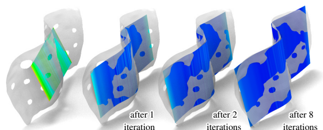
Fig. 11. A simple approximation problem, where a reference shape (point cloud) is approximated by a developable strip. The equations we use to express proximity make the strip grow so as to cover as much of the reference shape as possible. The number of iterations refers to guided projection according to § 3.2.
