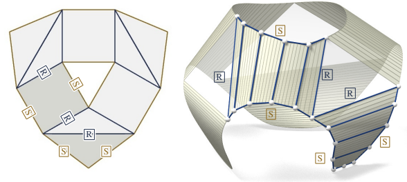
Fig. 5. The combinatorial setup of a composite seamless developable is stored in a mesh, where edges are labelled either \boxed{\text{R}} for “ruling” or \boxed{\text{S}} for “spline”. Faces accordingly correspond to spline developables, cones, or planar parts. The example shown here has no cones. There is smooth transition between surfaces along all nine \boxed{\text{R}} -edges, and between boundary curves in all 12 vertices.
