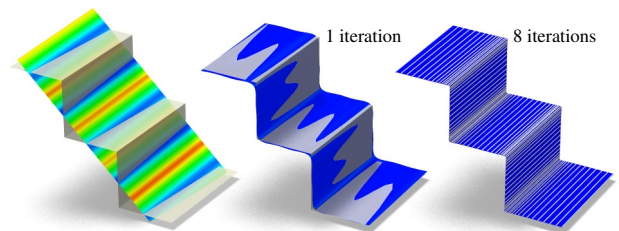
Fig. 16. Spline developables can approximate shapes with edges, if the normal spline is not enforced to have higher order smoothness and if \mathbf{n}(u_j) in (11) is considered fixed in each iteration of constraint solving. This image colour codes the distance of a developable spline strip from the reference shape.
