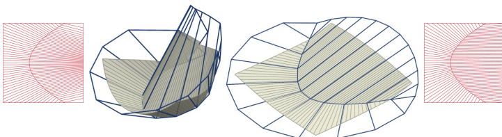
Fig. 13. Folding paper along a curved crease, maintaining isometry to the original rectangular shape, and maintaining the crease. In this case decomposition of the developable into smooth simple ruled pieces is not the most efficient way of computational handling of the problem. Instead we embed this model into a bigger surface which consists of two ruled strips and which develops onto a disk (the control net of the bigger surface is shown).
