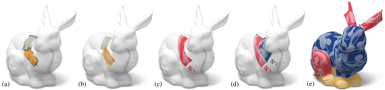
Fig. 10. Covering a complex shape by developable strips. (a) The user marks two areas on the bunny intended to be approximated by cubic developables. PCA is used to fit initial flat strips, which are visualized as rectangles. (b) The result of approximation. (c) The two strips obtained in the previous step are merged by putting together their respective control point sequences (averaging the end control points) and approximating again. (d) Having produced two strips side by side, they are subjected to the approximation procedure, with proximity of boundaries as an additional optimization goal. Such strips serve to initialize a composite surface. (e) The bunny is approximated by 6 composite surfaces shown in different colours. Figure 1 displays the same surface.
