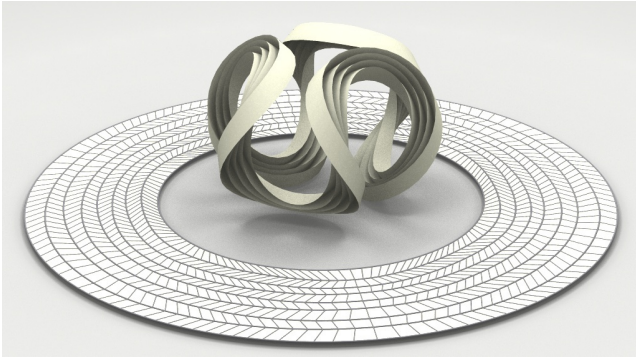
Fig. 12. This curved-crease sculpture is folded from an annulus. It has been interactively created along the lines of Figure 8. The annulus unfolding shown here actually is the mesh (\bar{V}, \bar{E}, \bar{F}) used for internal computations. Its edges correspond to creases and rulings.
