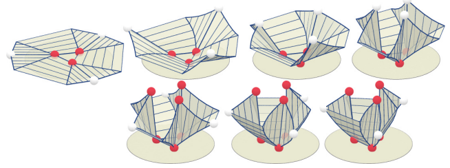
Fig. 8. Interactive modeling under curved-fold side conditions. Starting with a flat composite developable, on top we show dragging selected (white) vertices upwards while other vertices (red) remain fixed. The bottom row illustrates rotating selected vertices around a vertical axis. Control points are connected by blue edges.
