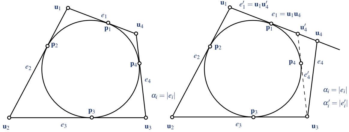
Figure 2: (a) A convex spherical quad having an incircle. This schematic illustration shows great circles as straight lines. (b) A convex spherical quad satisfying the angle criterion.
