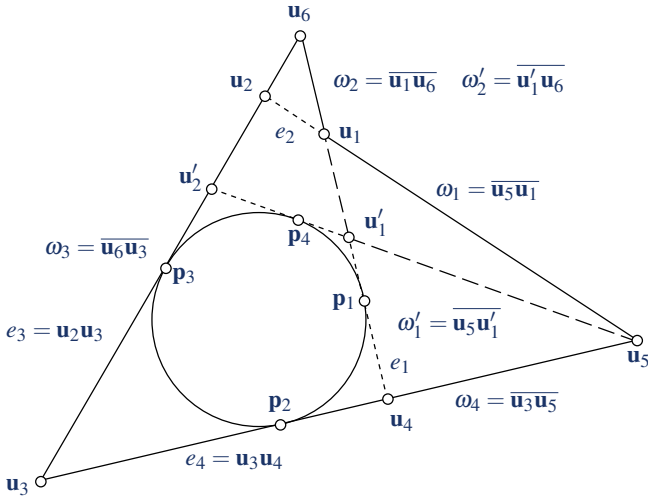
Figure 7: A parabolic admissible quad satisfying the angle criterion.
