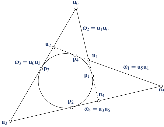
Figure 6: An admissible parabolic quad having an incircle.
