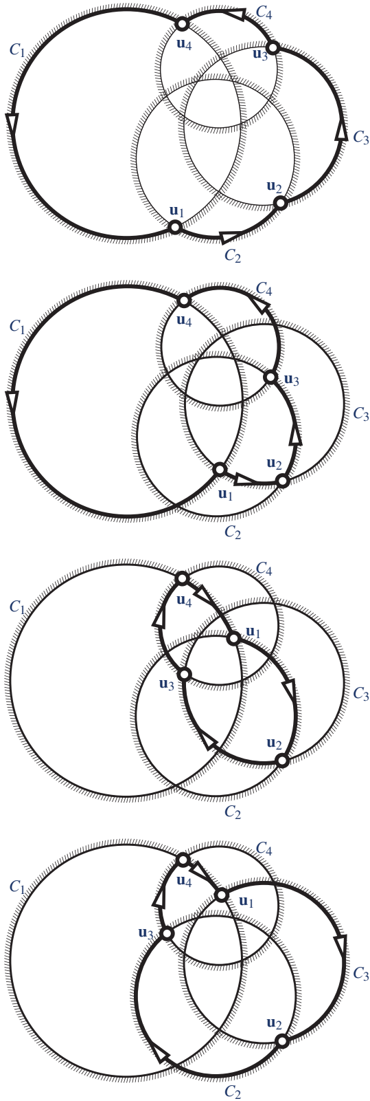
Figure 4: Stereographic images of four oriented great circles on the unit sphere. These four oriented circles correspond to four oriented planes incident with a vertex \mathbf{v} . The four figures show 4 of the total 12 admissible quads. Circle orientations are indicated by hatched boundaries.
