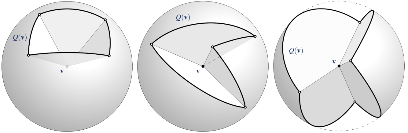
Figure 3: From left: elliptic, parabolic, and hyperbolic vertices, and their associated spherical quadrilaterals Q(\mathbf{v}) . The vertex \mathbf{v} is the center of the sphere.
