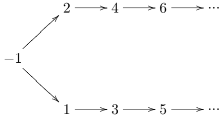
FIGURE 5.2. The Fibonacci tree
