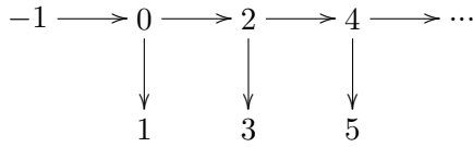
FIGURE 5.4. The comb tree
