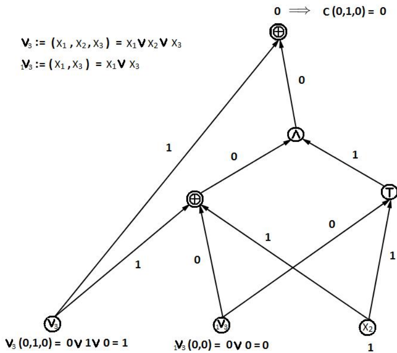
Figure A.3: Circuit and evaluation for input (0, 1, 0). For the definition of the used functions see Appendix A.1
