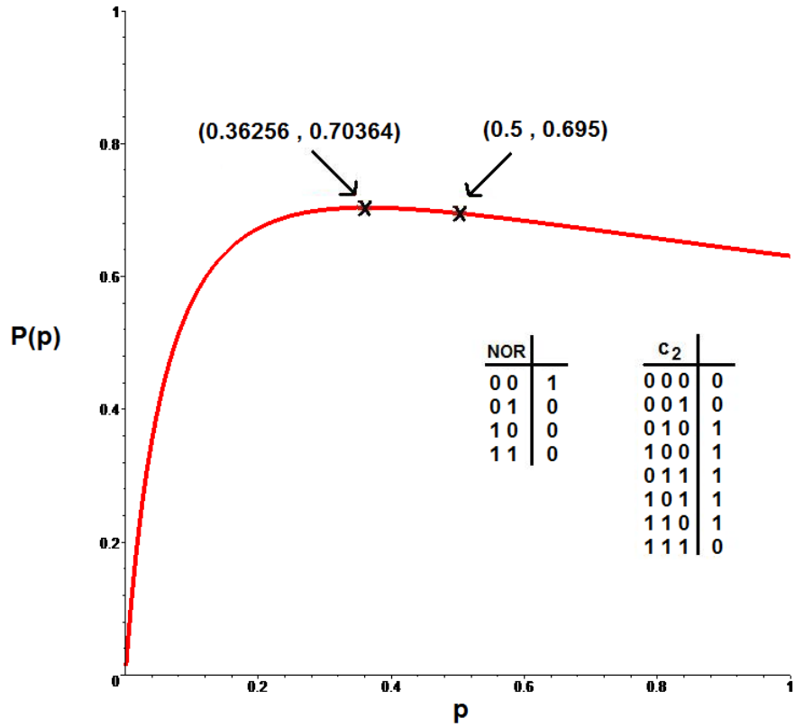
Figure 4.6: Non monotonous function P(p) with two connectors explained by their truth tables in the figure. The maximum of P(p) is at p^* \approx 0.36256
