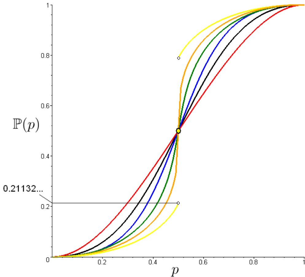
Figure 5.1: P(p) for different models: yellow: q = 0.6 , orange: q = 0.5 , green: q = 0.4 , black: q = 0 , blue: corresponding model of Yashunskii, red: F(p, p, p) . The function P(p) is approximated on the uniform grid with mesh-width 1/1000 where for each point 1000 iterations are performed (the blue and the red curves are exact).
