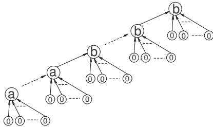
Figure 8: A tree T of type \text{I}^{[K]} .
