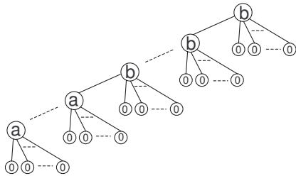
Figure 6: A tree T of type I^{[P]} .
