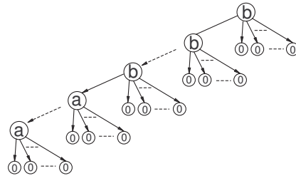
Figure 9: A tree T of type \text{II}^{[K]} .
