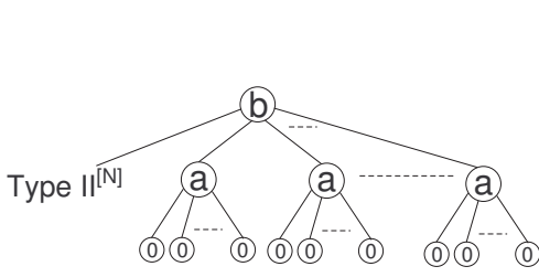
Figure 4: A tree T of type I^{[N]} .
