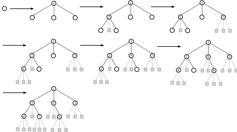
Figure 4: An illustration of the recursive construction of a ternary increasing trees, with respect to the path diagram (\lambda(u), s) with \lambda(u) = v = a_{0,2} a_{2,1}^{(2)} b_3 b_2 c_1^{(3)} b_1 and s = 0030011
