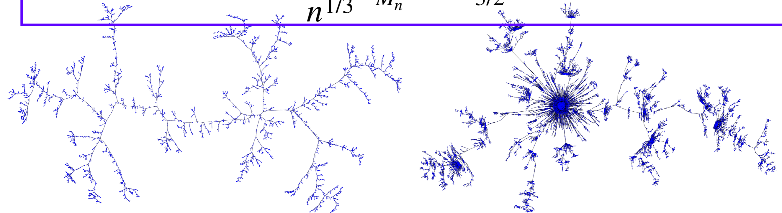
Brownian Tree \mathcal{T}_2
